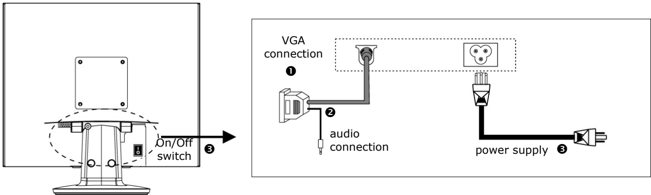
(III.: Rearside connectors)
